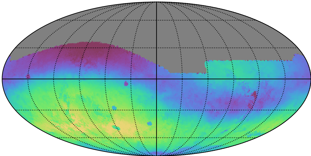
too_ignore_5_4v3.4_10yrs All sky g band: Median skyBrightness
