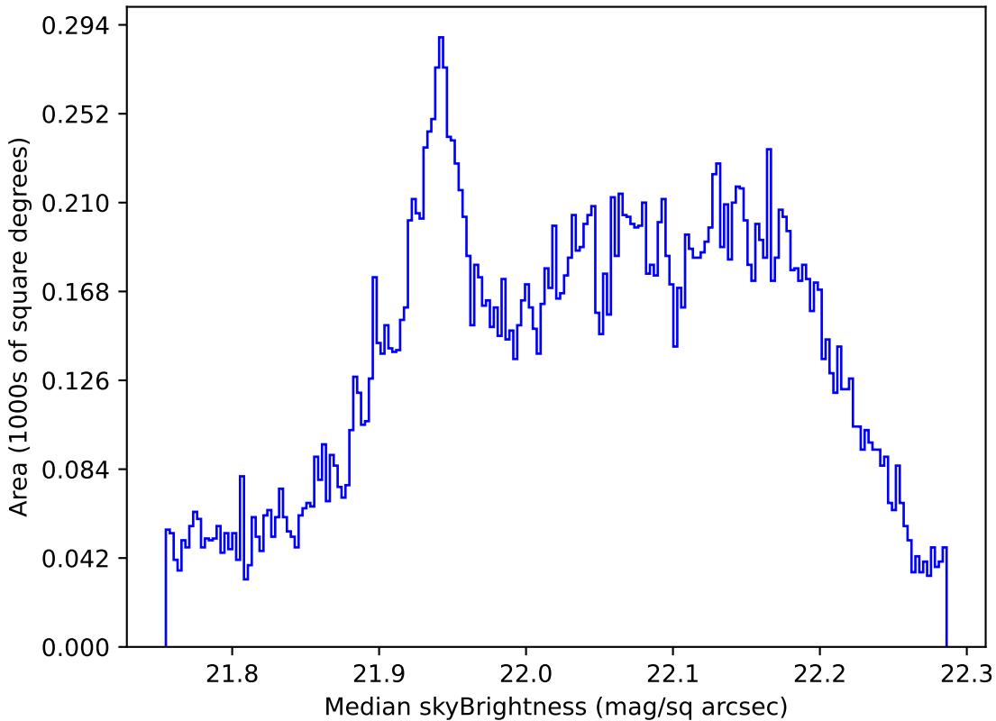
too_ignore_5_4v3.4_10yrs All sky g band: Median skyBrightness
