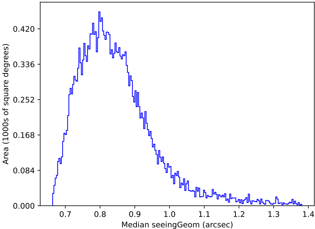
too_ignore_5_4v3.4_10yrs Yr 1 z band: Median seeingGeom
