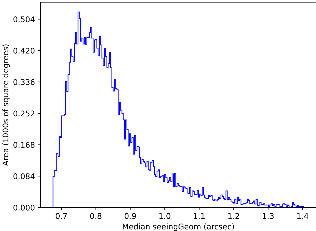
too_ignore_5_4v3.4_10yrs Yr 1 i band: Median seeingGeom
