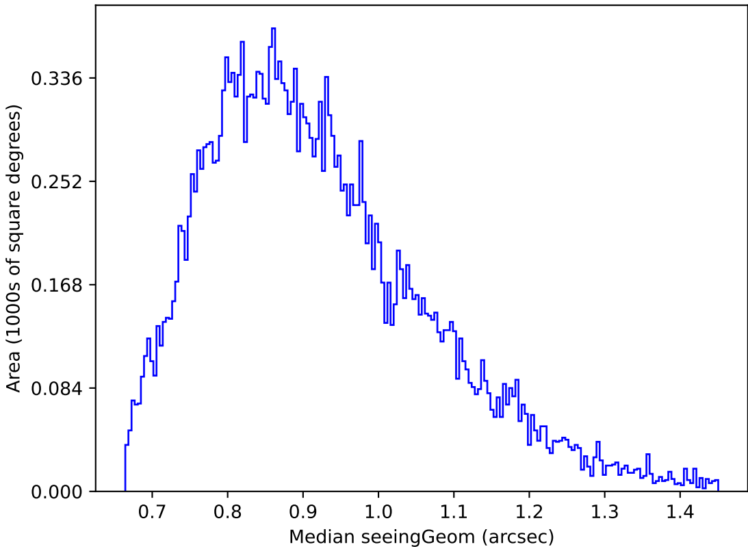
too_ignore_5_4v3.4_10yrs Yr 1 g band: Median seeingGeom
