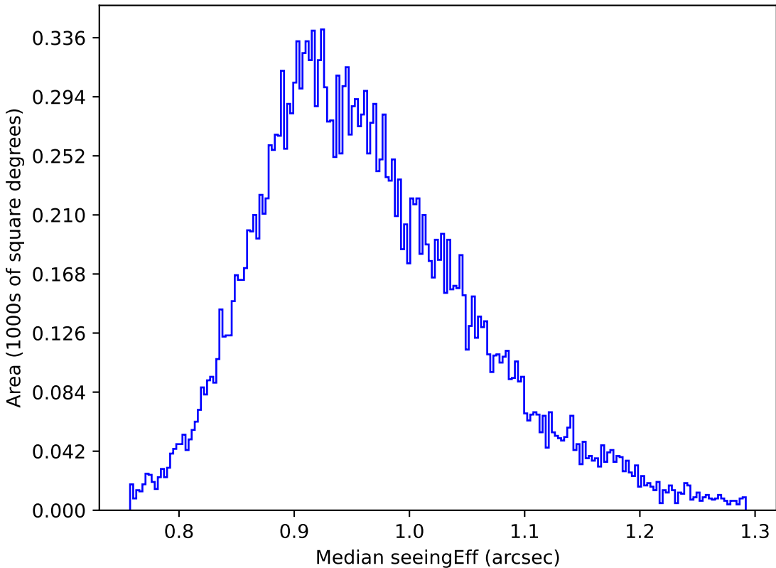
too_ignore_5_4v3.4_10yrs Yr 1 y band: Median seeingEff
