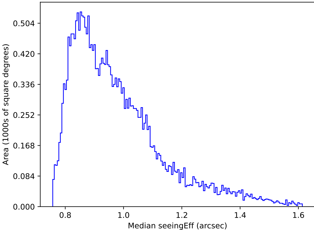
too_ignore_5_4v3.4_10yrs Yr 1 r band: Median seeingEff
