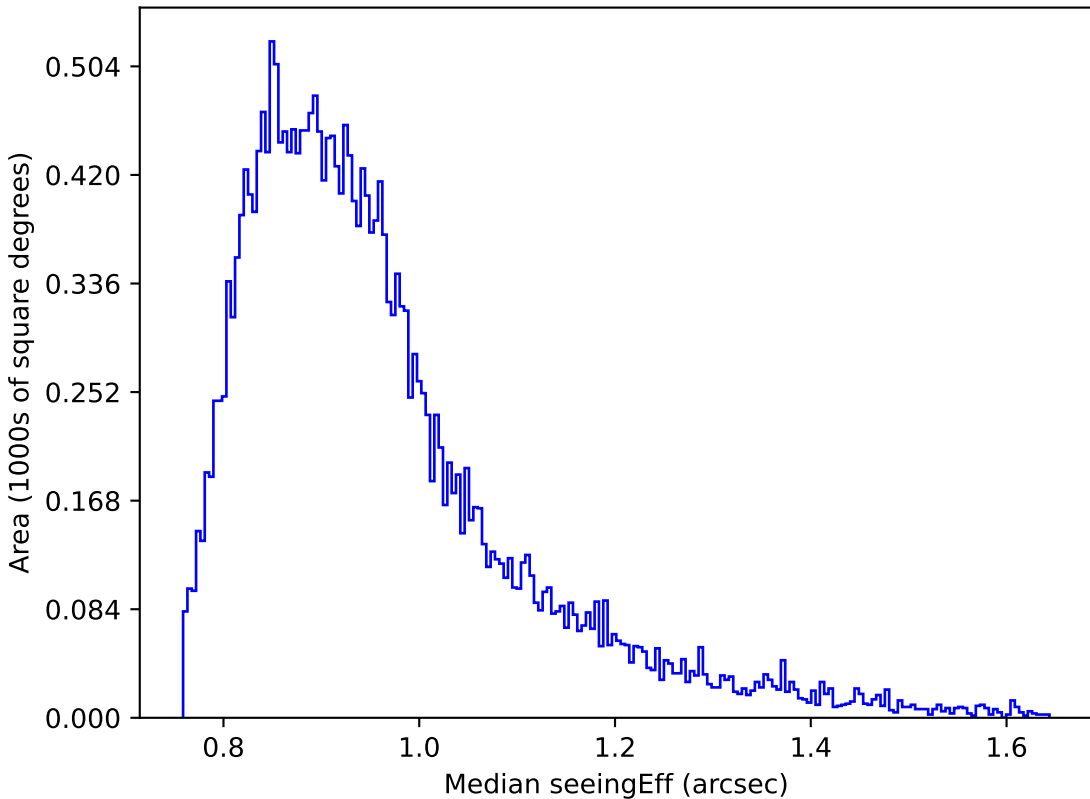
too_ignore_5_4v3.4_10yrs Yr 1 i band: Median seeingEff
