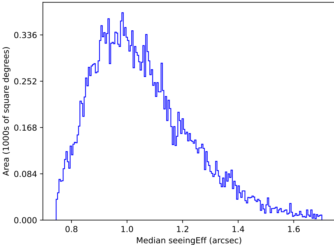
too_ignore_5_4v3.4_10yrs Yr 1 g band: Median seeingEff
