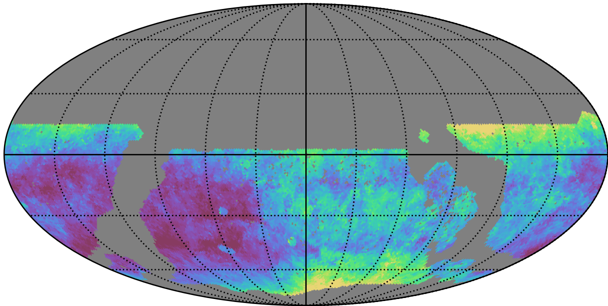
too_ignore_5_4v3.4_10yrs WFD z band: Median seeingEff
