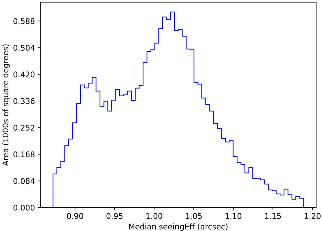
too_ignore_5_4v3.4_10yrs WFD z band: Median seeingEff
