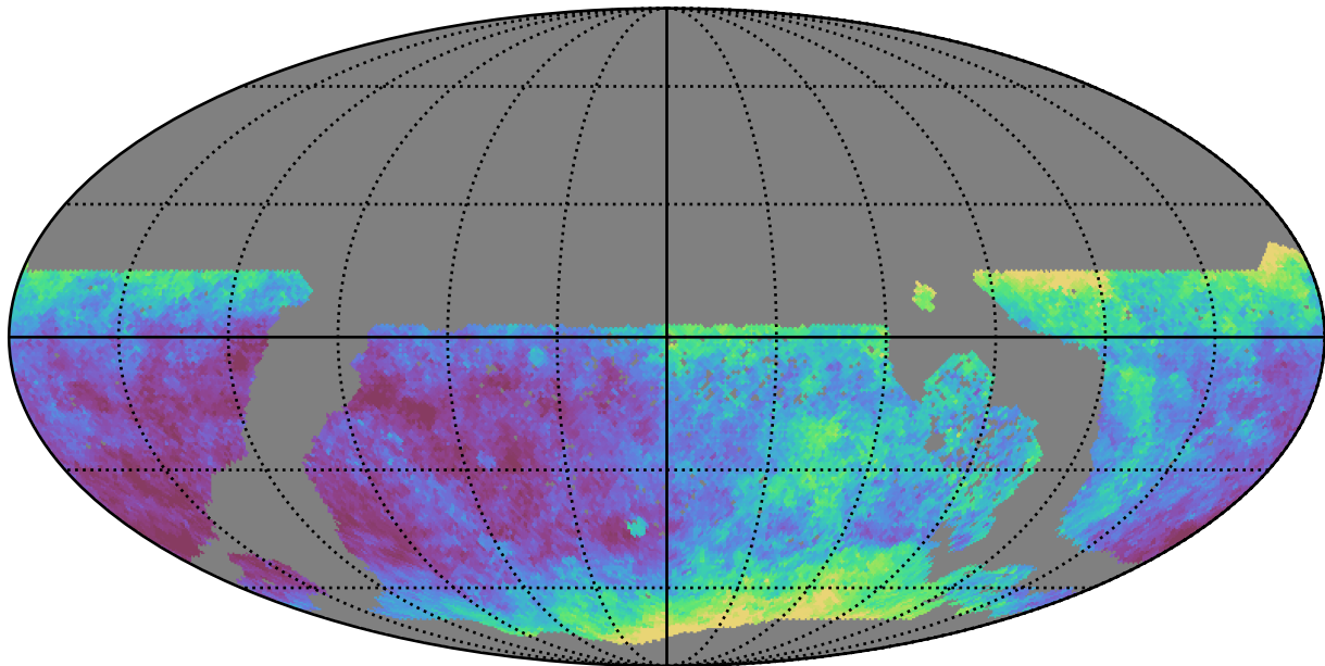
too_ignore_5_4v3.4_10yrs WFD y band: Median seeingEff
