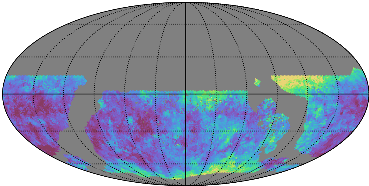
too_ignore_5_4v3.4_10yrs WFD u band: Median seeingEff
