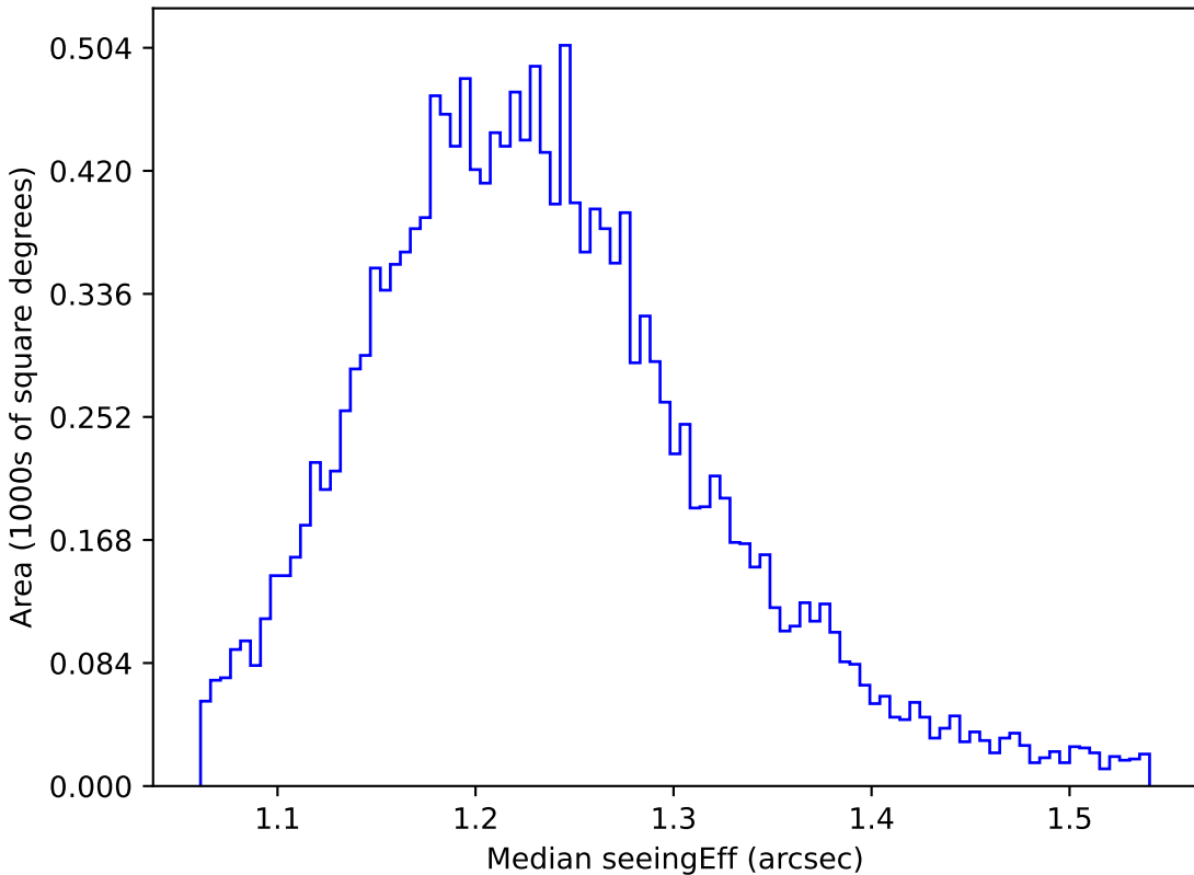
too_ignore_5_4v3.4_10yrs WFD u band: Median seeingEff
