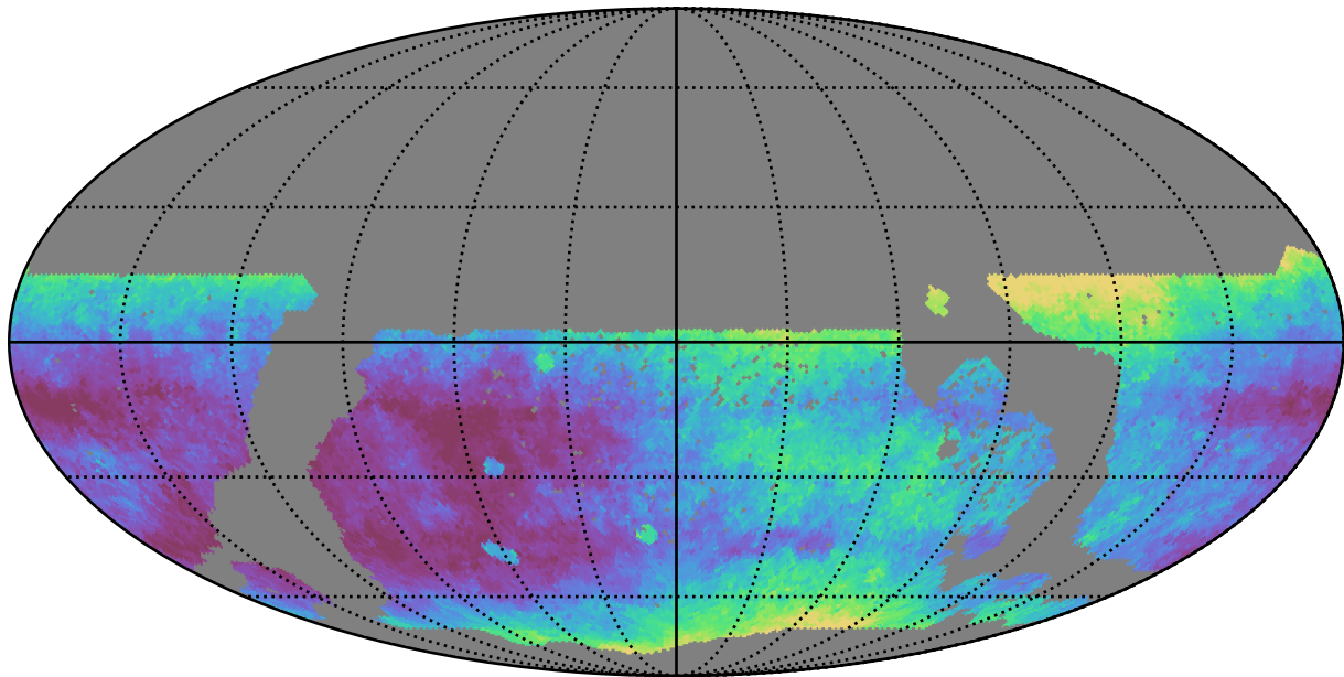
too_ignore_5_4v3.4_10yrs WFD r band: Median seeingEff
