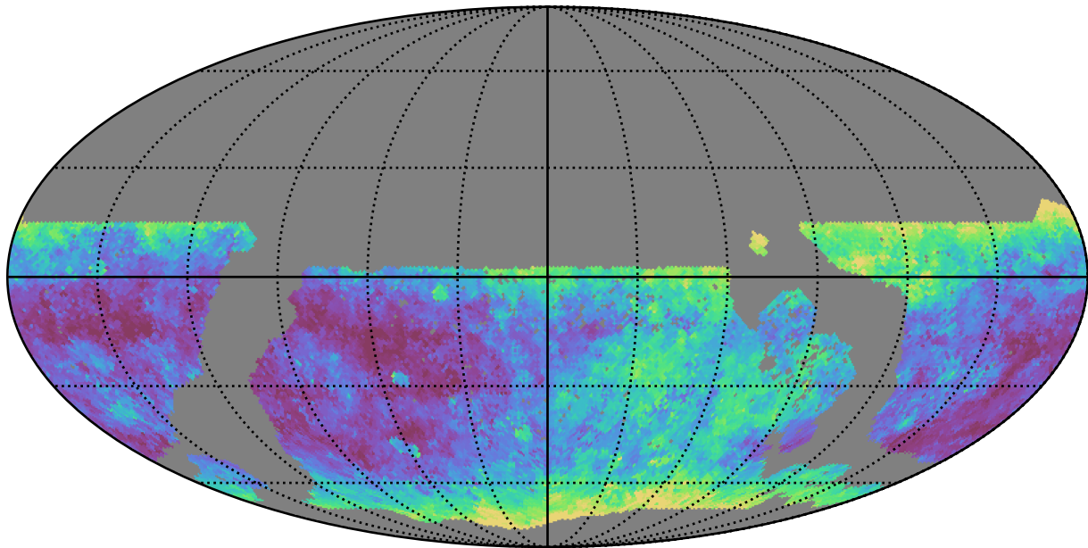
too_ignore_5_4v3.4_10yrs WFD g band: Median seeingEff
