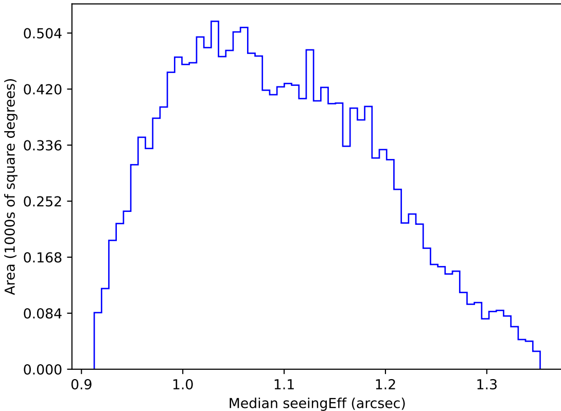
too_ignore_5_4v3.4_10yrs WFD g band: Median seeingEff
