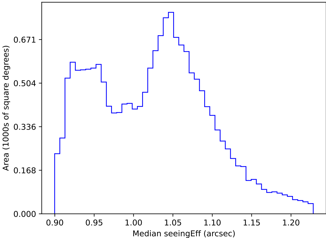
too_ignore_5_4v3.4_10yrs WFD all bands: Median seeingEff
