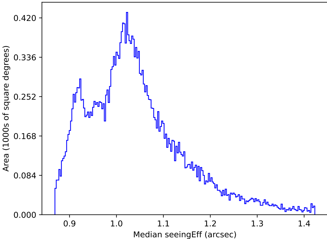
too_ignore_5_4v3.4_10yrs All sky z band: Median seeingEff
