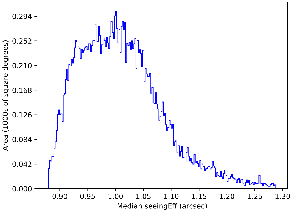
too_ignore_5_4v3.4_10yrs All sky y band: Median seeingEff
