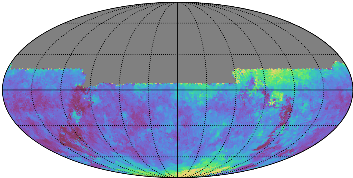
too_ignore_5_4v3.4_10yrs All sky u band: Median seeingEff
