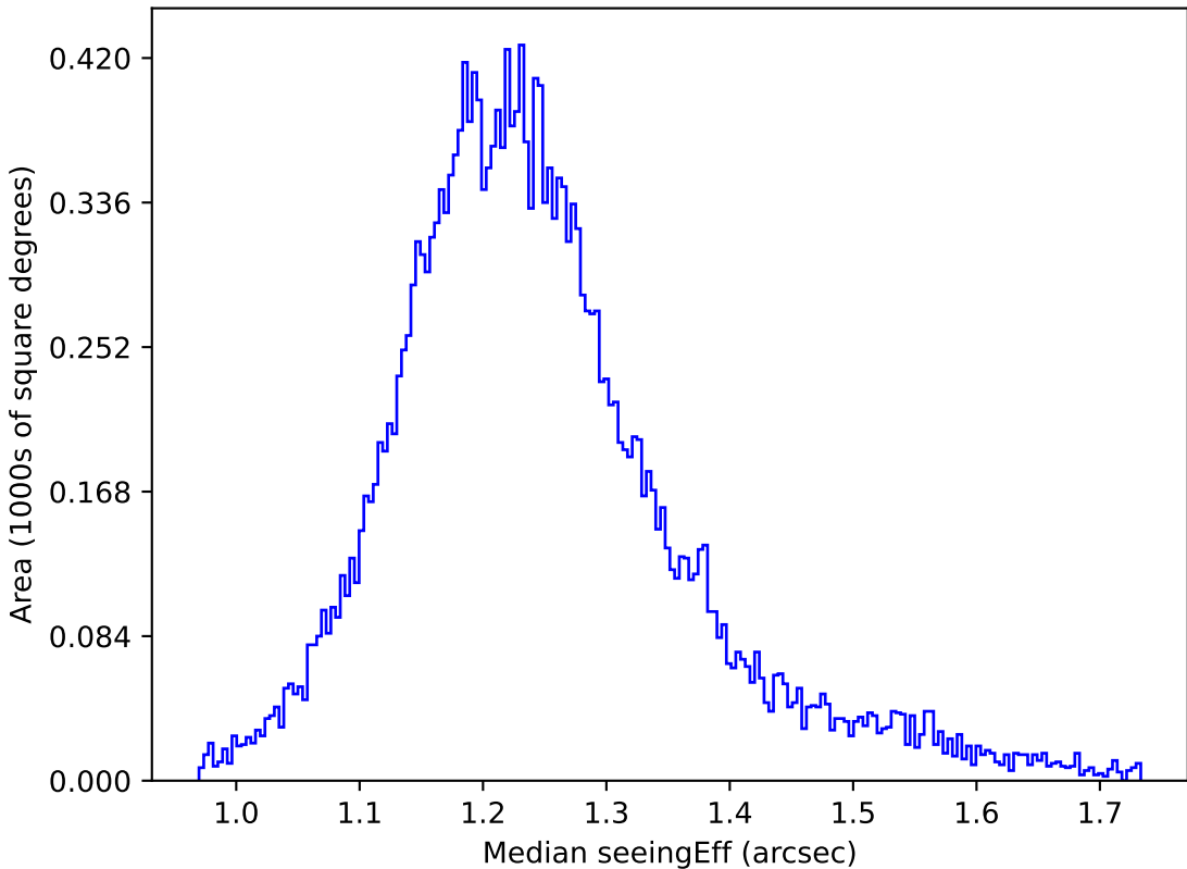
too_ignore_5_4v3.4_10yrs All sky u band: Median seeingEff
