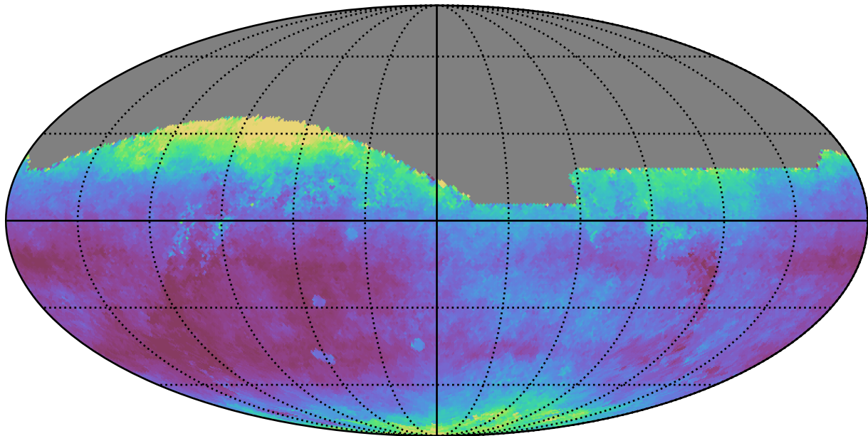
too_ignore_5_4v3.4_10yrs All sky r band: Median seeingEff
