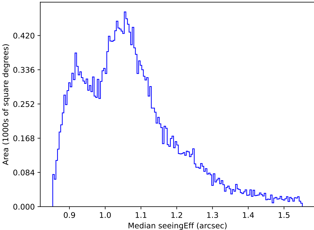
too_ignore_5_4v3.4_10yrs All sky r band: Median seeingEff
