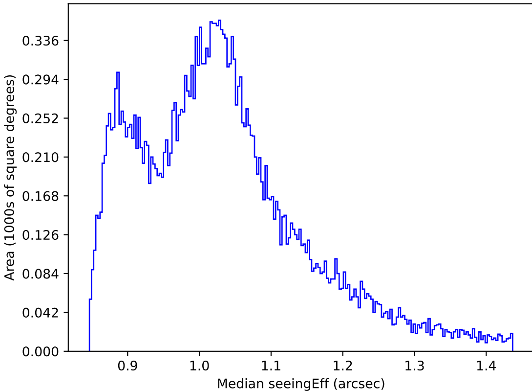
too_ignore_5_4v3.4_10yrs All sky i band: Median seeingEff
