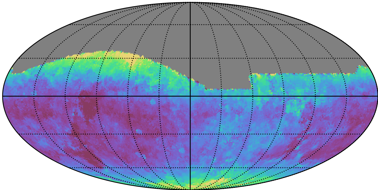
too_ignore_5_4v3.4_10yrs All sky g band: Median seeingEff
