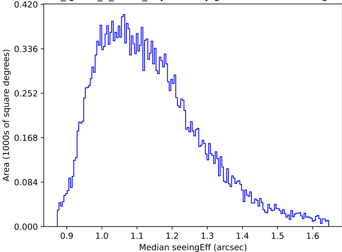
too_ignore_5_4v3.4_10yrs All sky g band: Median seeingEff
