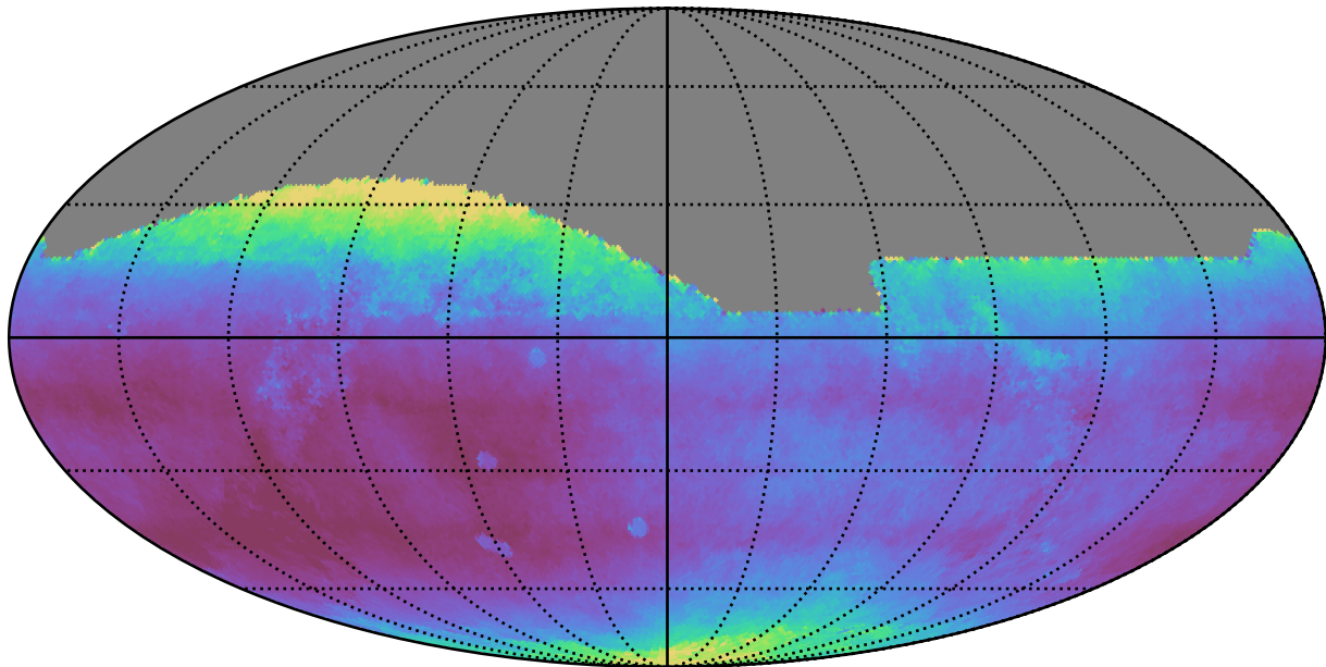
too_ignore_5_4v3.4_10yrs All sky all bands: Median seeingEff
