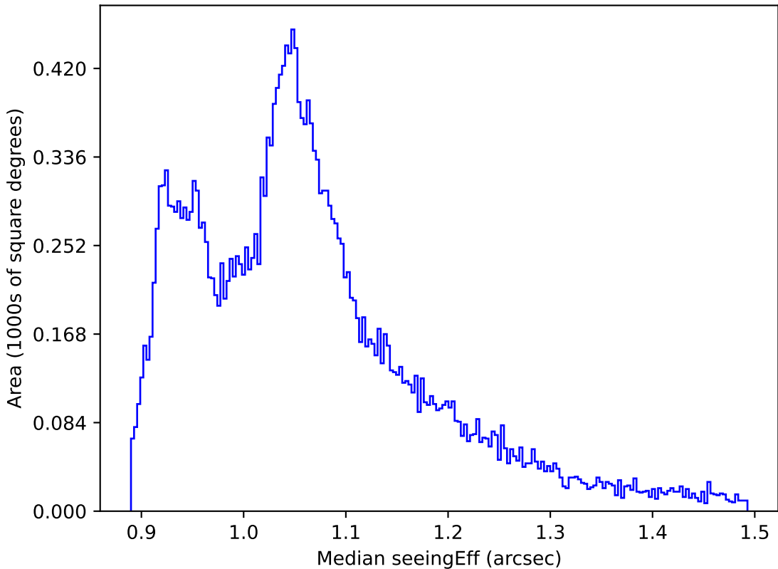
too_ignore_5_4v3.4_10yrs All sky all bands: Median seeingEff
