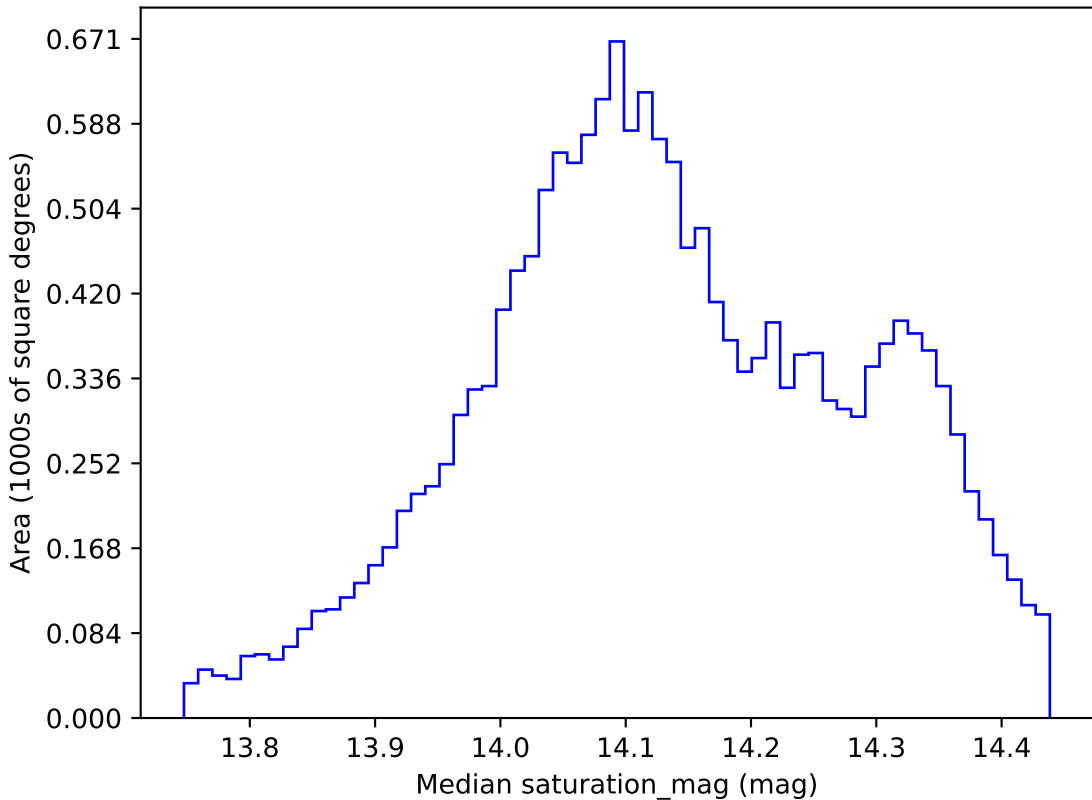
too_ignore_5_4v3.4_10yrs WFD z band: Median saturation_mag
