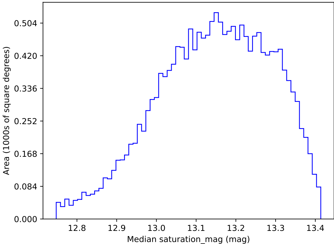
too_ignore_5_4v3.4_10yrs WFD y band: Median saturation_mag
