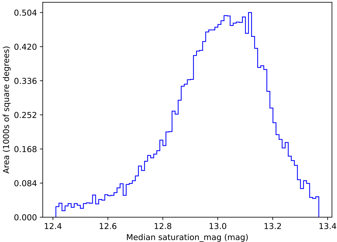
too_ignore_5_4v3.4_10yrs WFD u band: Median saturation_mag
