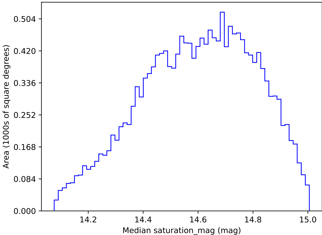
too_ignore_5_4v3.4_10yrs WFD g band: Median saturation_mag
