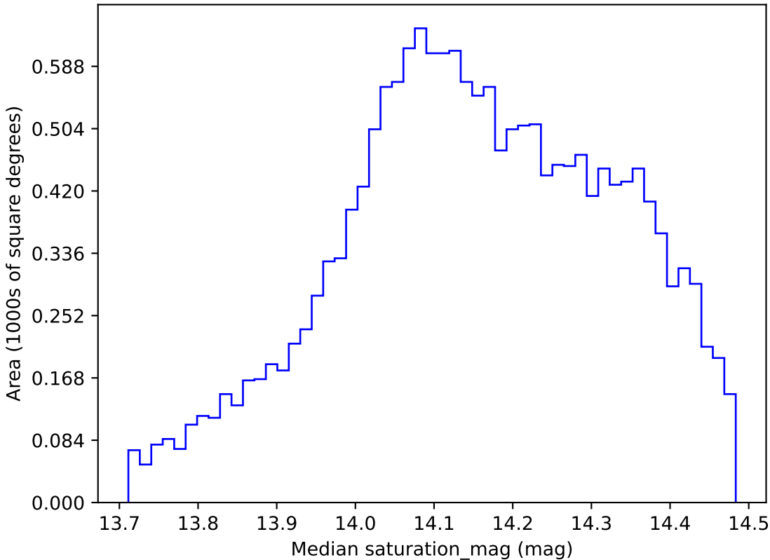
too_ignore_5_4v3.4_10yrs WFD all bands: Median saturation_mag
