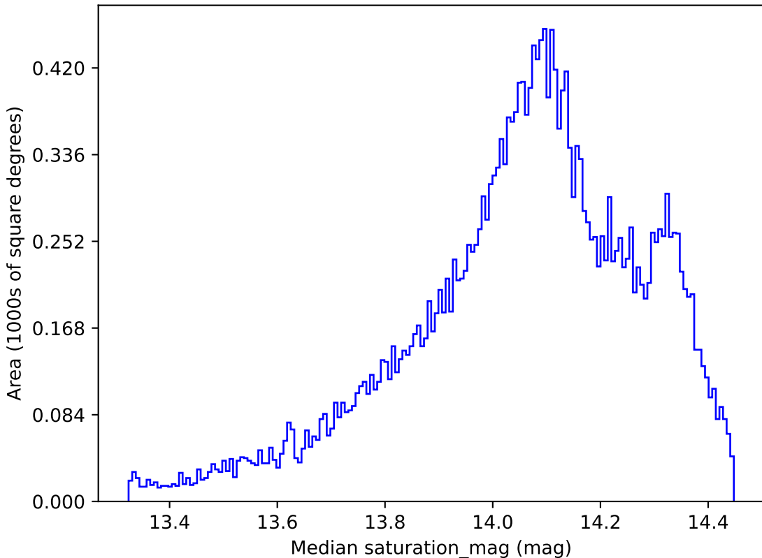
too_ignore_5_4v3.4_10yrs All sky z band: Median saturation_mag
