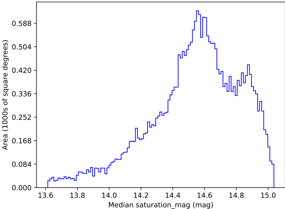
too_ignore_5_4v3.4_10yrs All sky r band: Median saturation_mag
