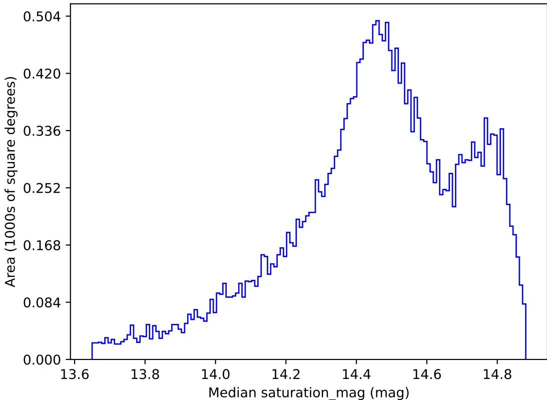
too_ignore_5_4v3.4_10yrs All sky i band: Median saturation_mag
