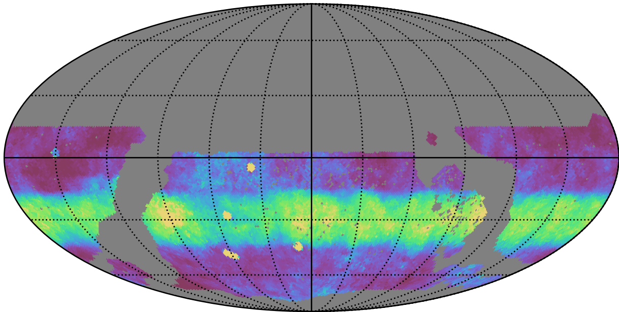
too_ignore_5_4v3.4_10yrs WFD z band: Median normairmass
