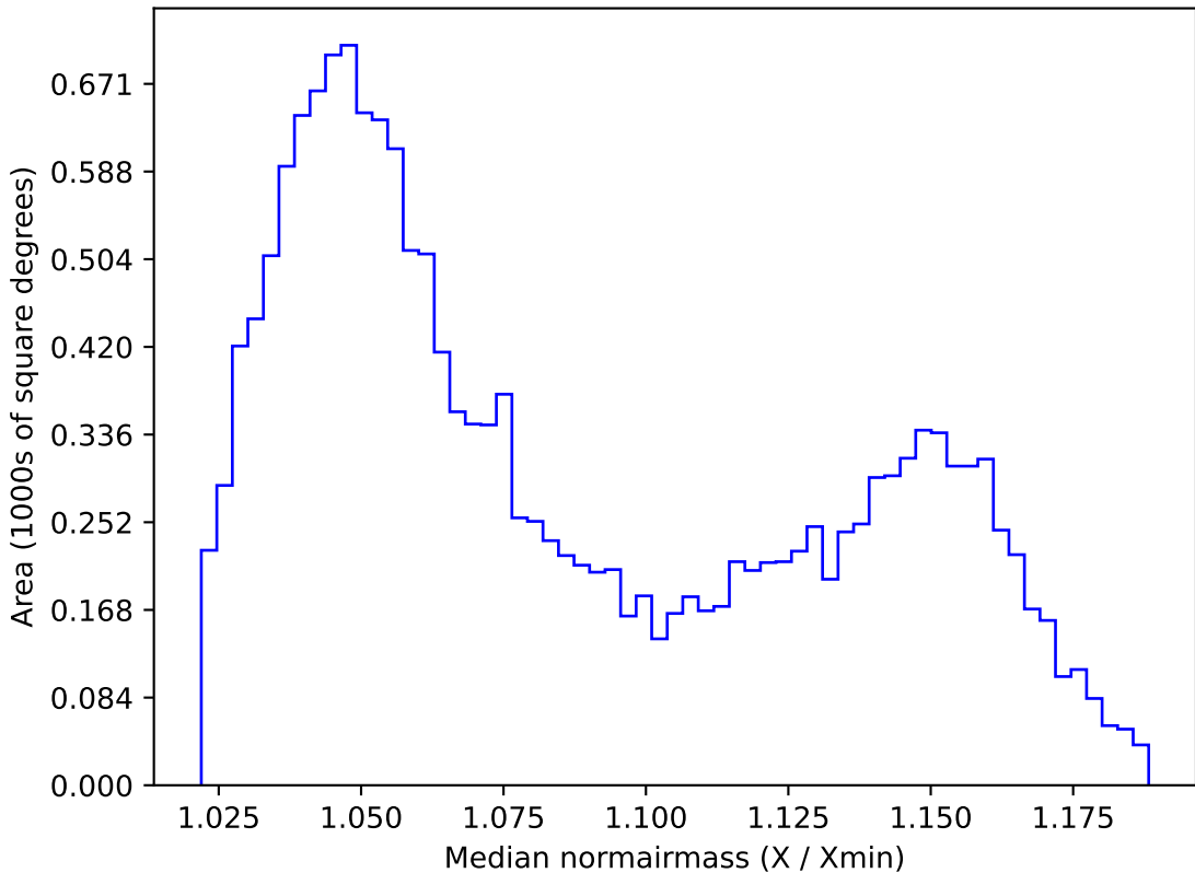
too_ignore_5_4v3.4_10yrs WFD z band: Median normairmass
