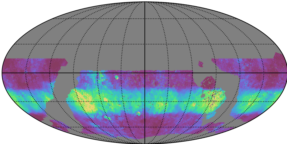
too_ignore_5_4v3.4_10yrs WFD u band: Median normairmass
