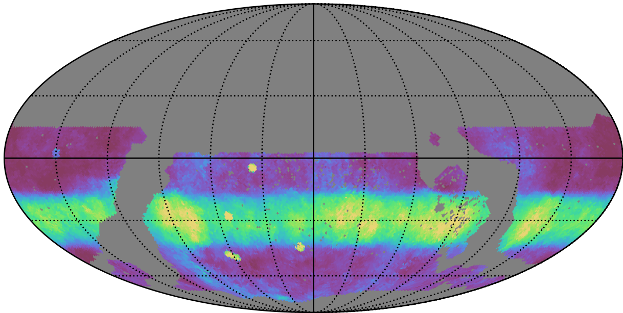
too_ignore_5_4v3.4_10yrs WFD r band: Median normairmass
