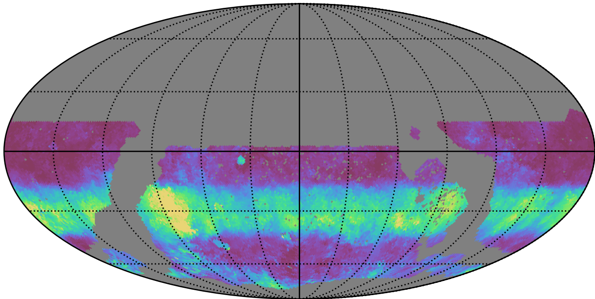
too_ignore_5_4v3.4_10yrs WFD g band: Median normairmass
