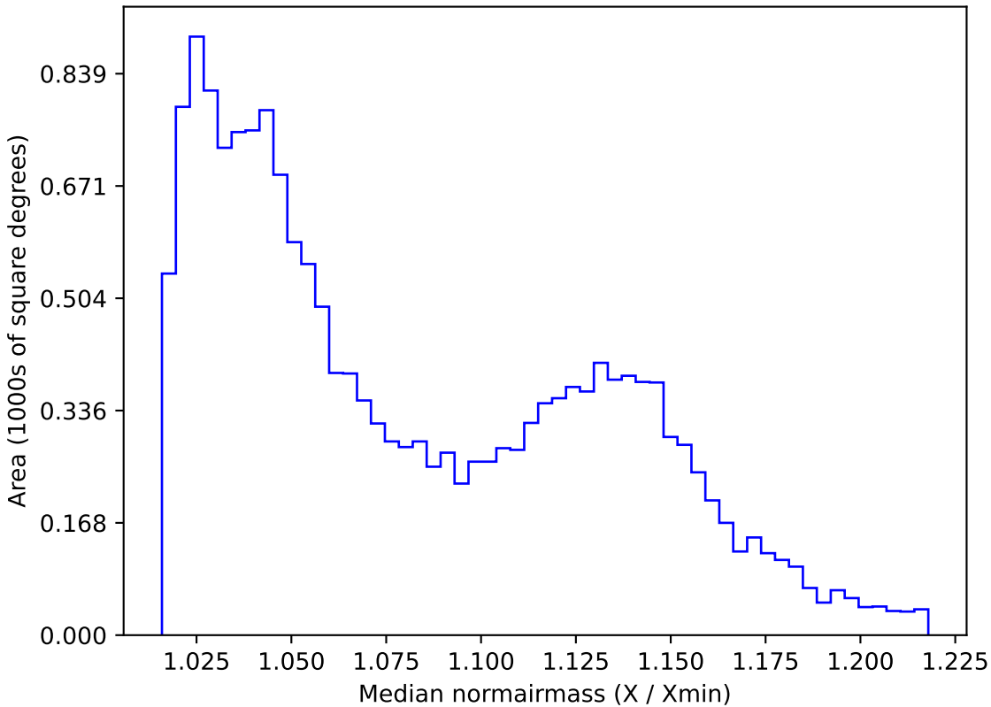
too_ignore_5_4v3.4_10yrs WFD g band: Median normairmass
