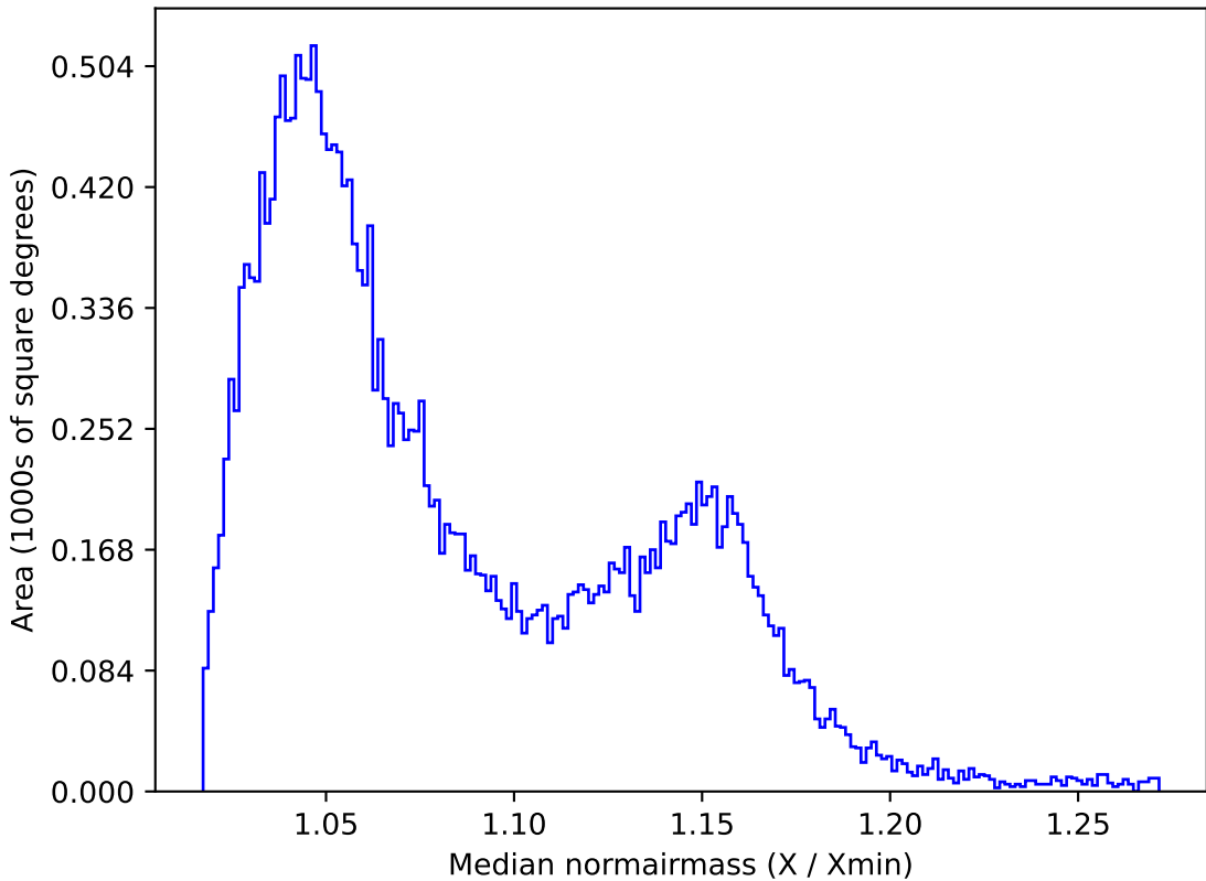
too_ignore_5_4v3.4_10yrs All sky z band: Median normairmass
