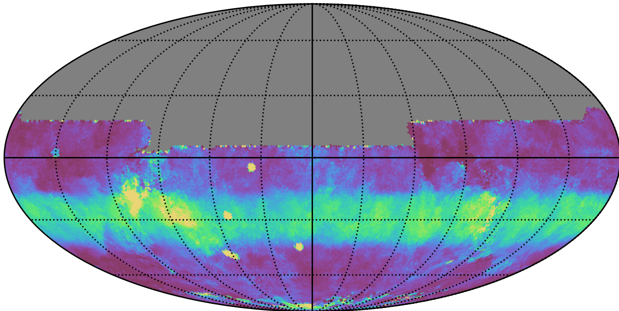
too_ignore_5_4v3.4_10yrs All sky y band: Median normairmass
