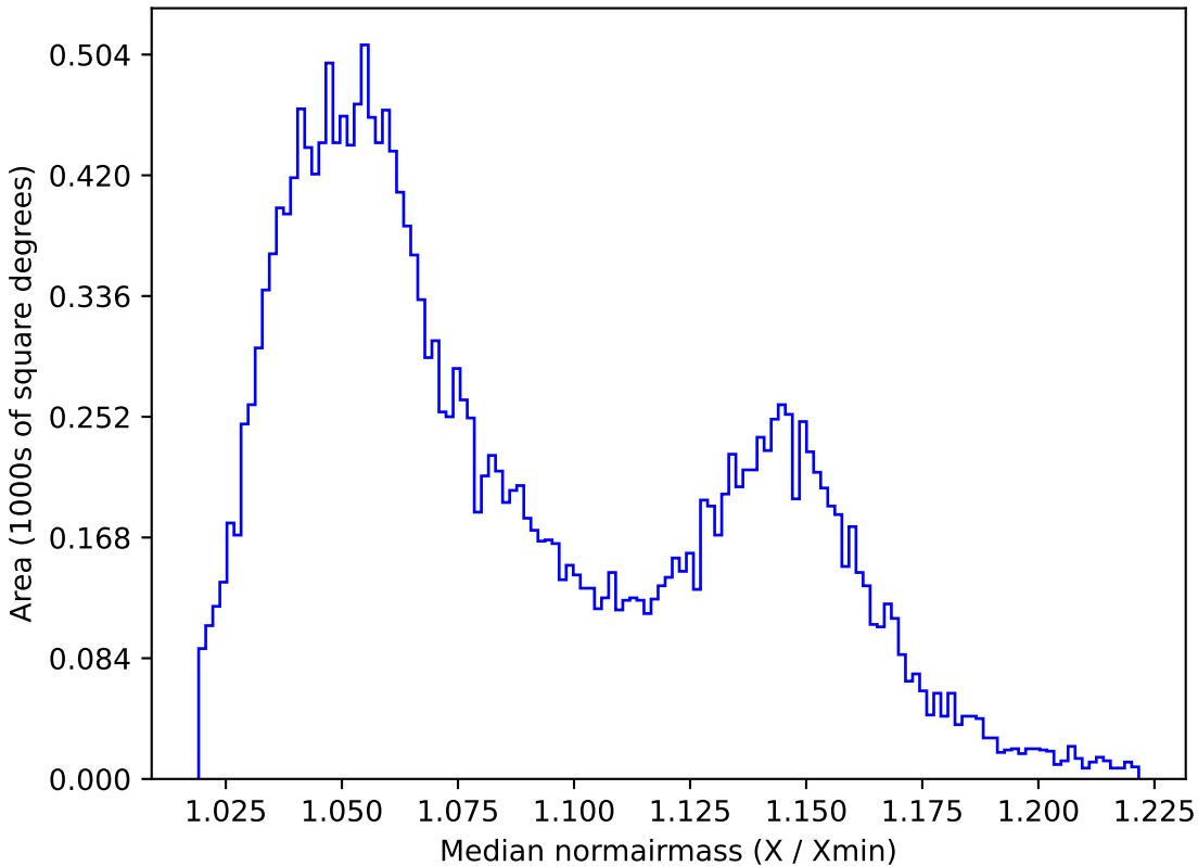
too_ignore_5_4v3.4_10yrs All sky y band: Median normairmass
