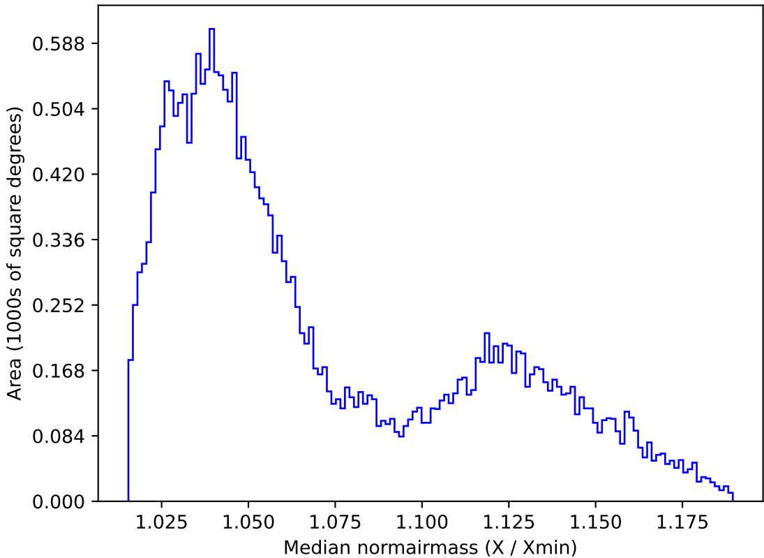
too_ignore_5_4v3.4_10yrs All sky r band: Median normairmass
