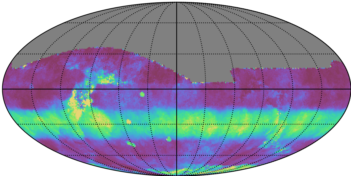
too_ignore_5_4v3.4_10yrs All sky i band: Median normairmass
