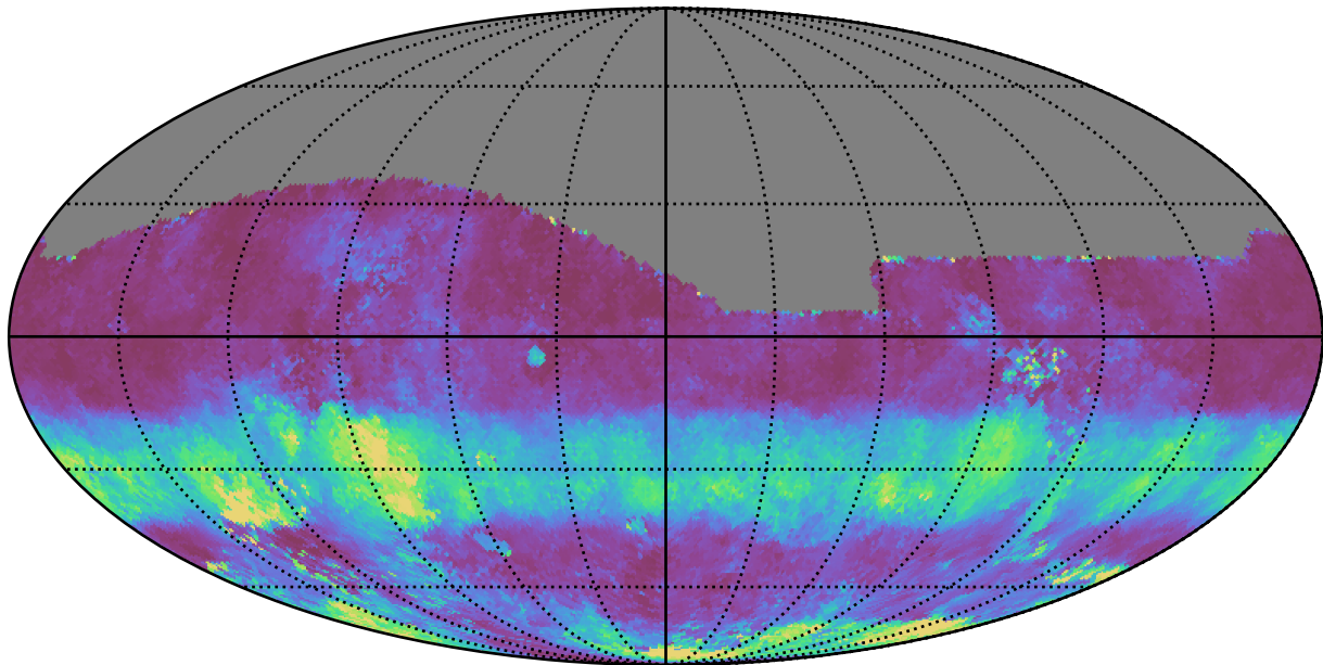
too_ignore_5_4v3.4_10yrs All sky g band: Median normairmass
