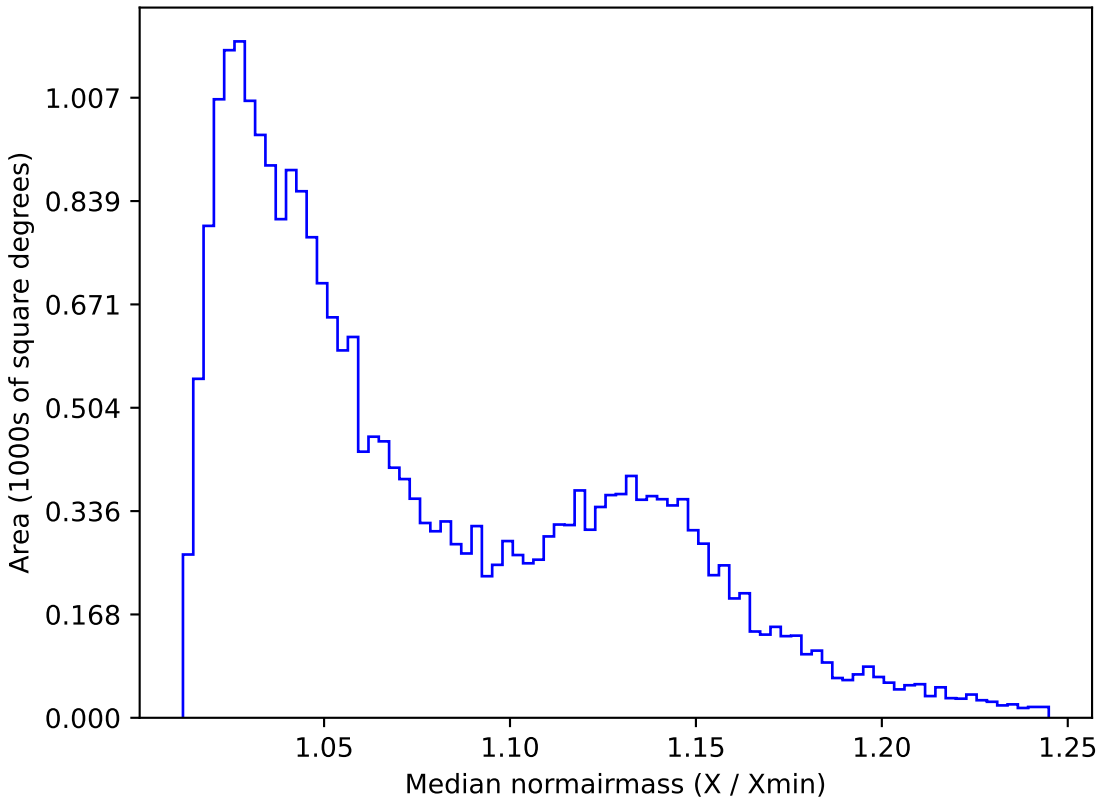
too_ignore_5_4v3.4_10yrs All sky g band: Median normairmass
